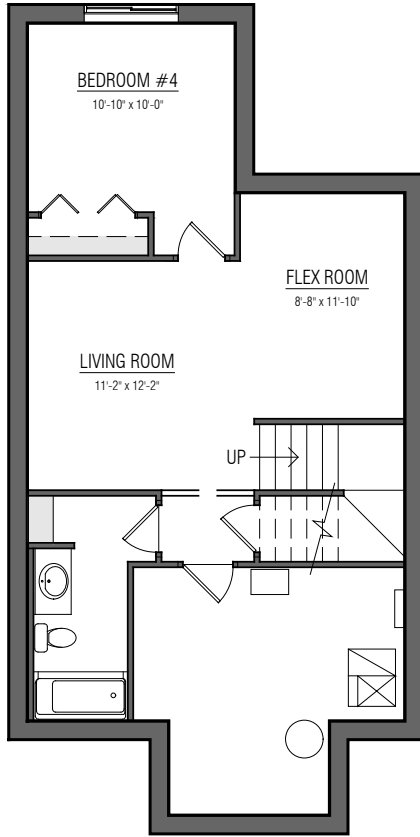
OPTION #1 - 540 SQ.FT.
