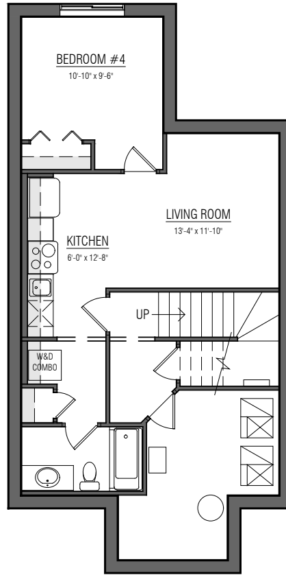
OPTION #1 - 580 SQ.FT.
