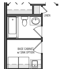
LAUNDRY ROOM WITH SINK & LINEN CLOSET
