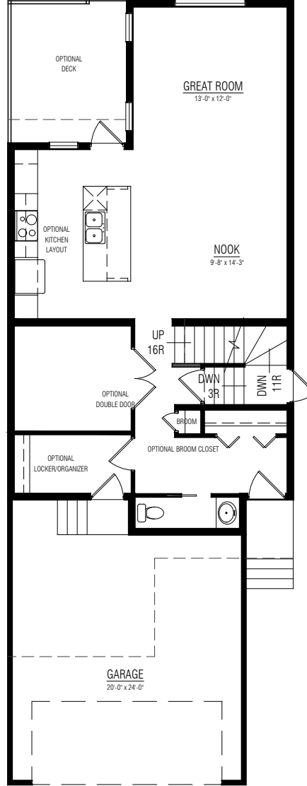
MAIN FLOOR OPTION LARGER KITCHEN ISLAND & OPTIONAL DECK
