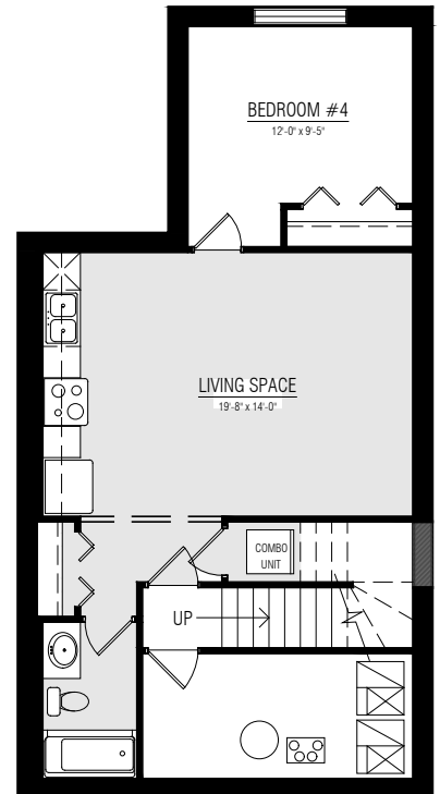
BASEMENT SUITE DEVELOPMENT OPTION 610 SQ. FT.
