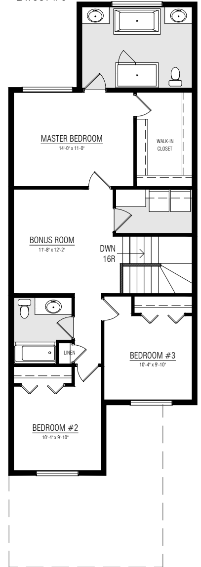
UPPER FLOOR OPTION ALTERNATE ENSUITE
