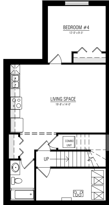
BASEMENT SUITE DEVELOPMENT 610 SQ. FT.
