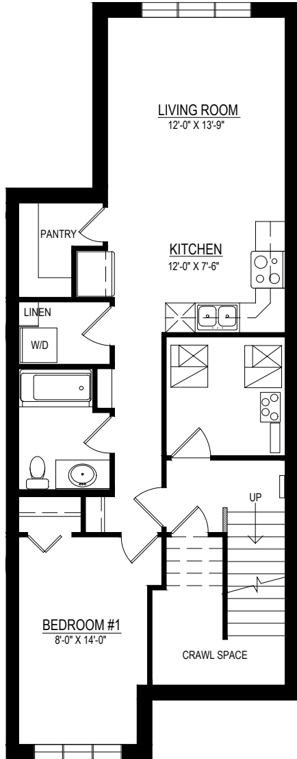
BASEMENT SUITE OPTION OPTION 1 616 SQ. FT.
