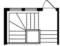
REAR STAIRWELL LOCATION OPTION ADDS 88 SQ. FT.
