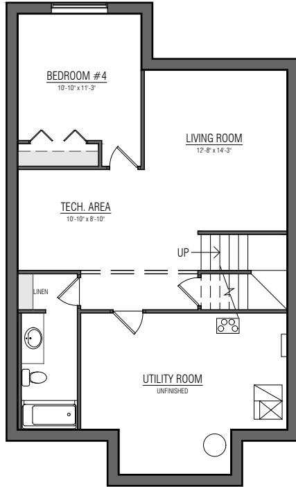
BASEMENT DEVELOPMENT 632 SQ. FT.
