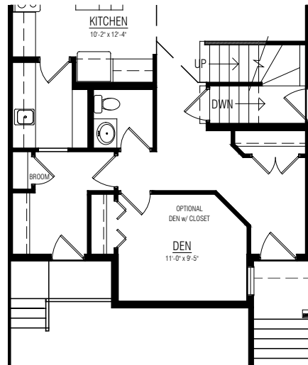
MAIN FLOOR OPTIONS BUTLER'S PANTRY
