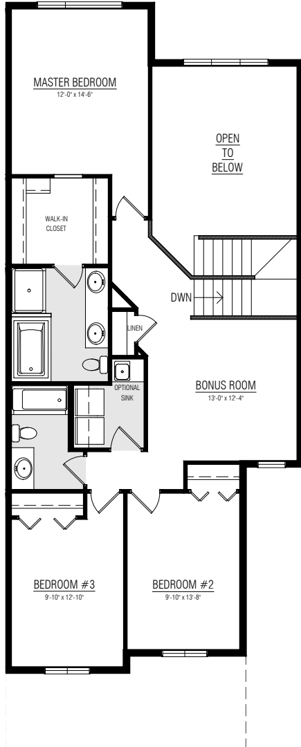
UPPER FLOOR STANDARD 1142 SQ. FT.
