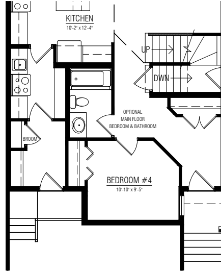
MAIN FLOOR OPTIONS SPICE KITCHEN
