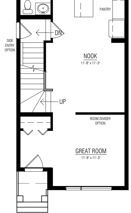
MAIN FLOOR OPTION ROOM DIVIDER
