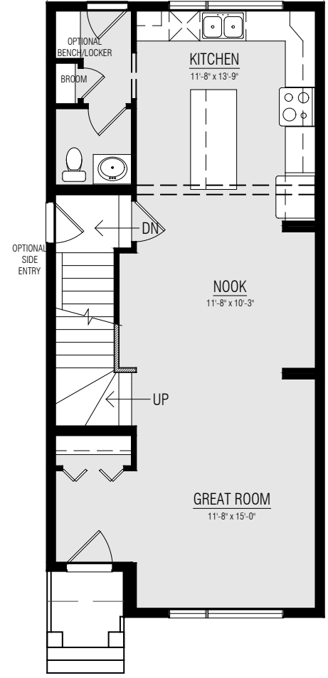
MAIN FLOOR OPTION REAR KITCHEN
