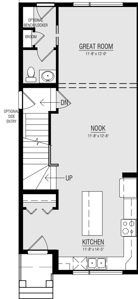
MAIN FLOOR OPTION FRONT KITCHEN
