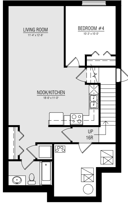
BASEMENT SUITE DEVELOPMENT 700 SQ. FT.
