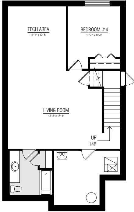
BASEMENT DEVELOPMENT 700 SQ. FT.
